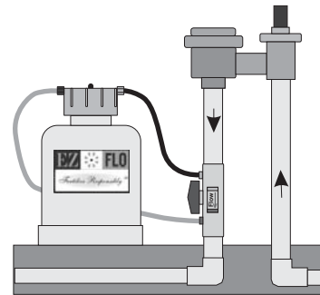
Sprinkler/Drip Connection
